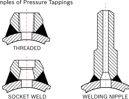
Examples of Pressure Tappings
